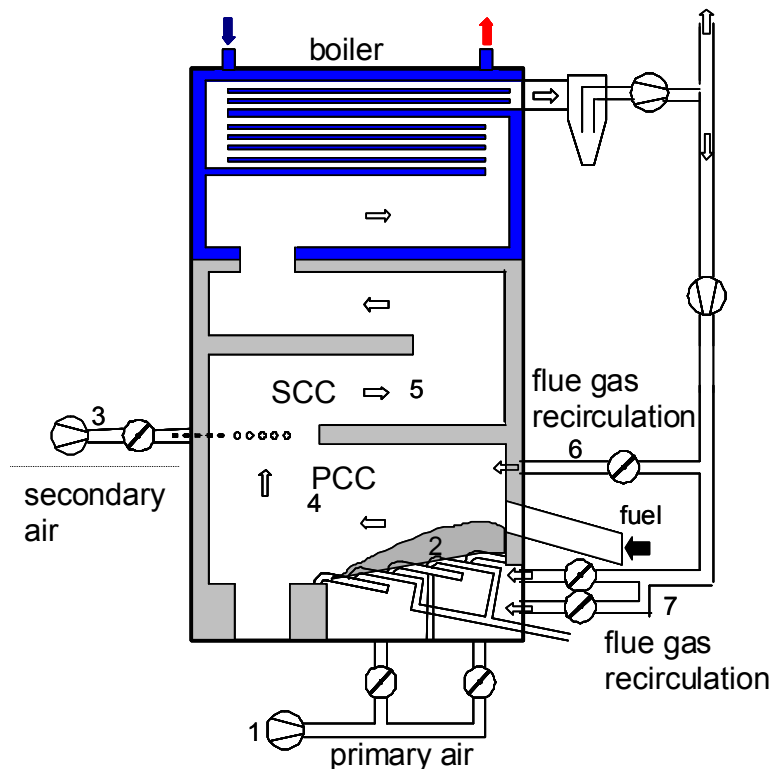
Figure 1: Scheme of a plant equipped with air staging technology
